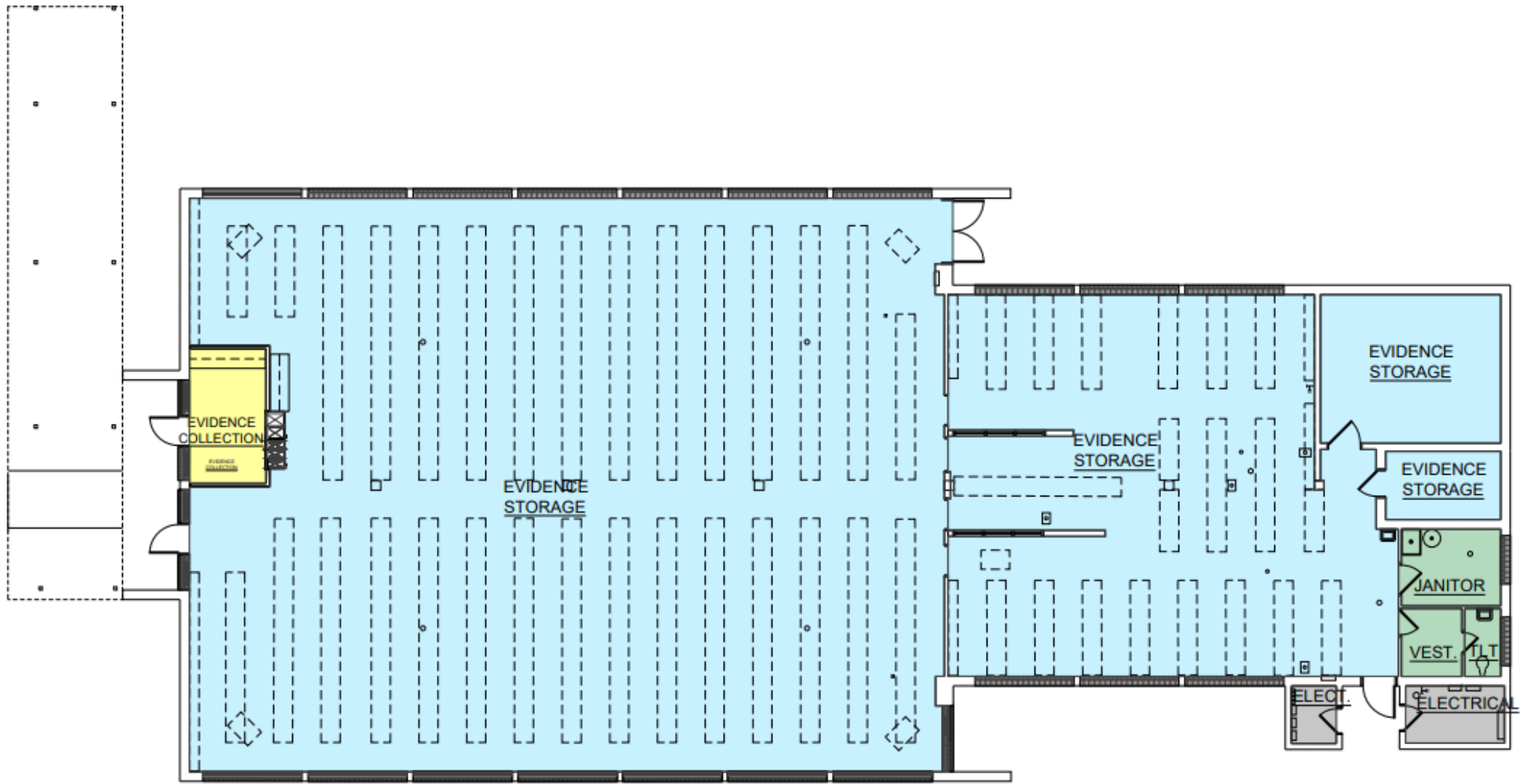
PROPOSED EVIDENCE STORAGE FLOOR PLAN
