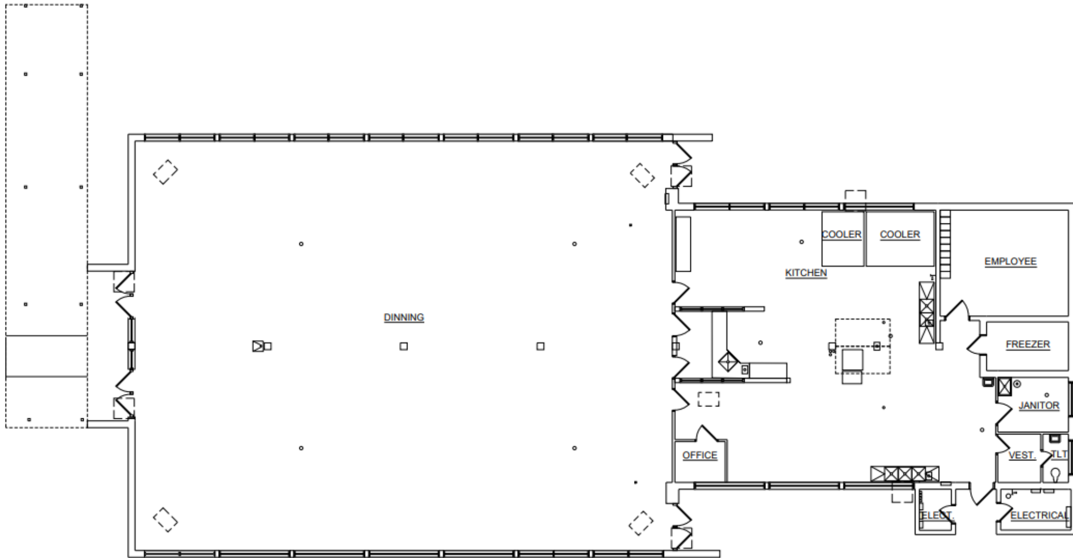
EXISTING CAFETERIA BUILDING FLOOR PLAN
